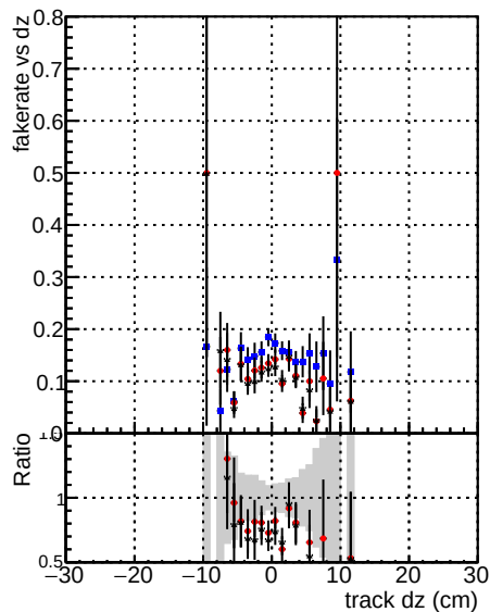
Configuration DOM V0001 R0000000001 Global CMSSW ckfPU50 RECO Fake rate vs d DOM V0001 R0000000001 Global CMSSW ckfPU50 RECO DOM V0001 R0000000001 Global CMSSW mkFitPU50LowPt Quad DOM V0001 R0000000001 Global CMSSW LowPtNonclean RECO
