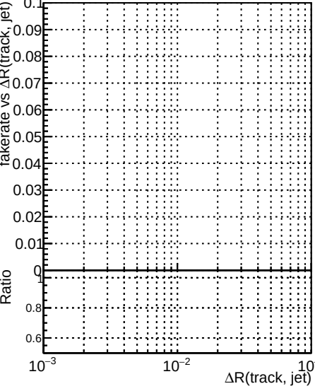
Fake rate vs ΔR(track, jet) —●— DQM_V0001_R000000001_Global_CMSSW_ckfPU50_RECO —●— DQM_V0001_R000000001_Global_CMSSW_mkFitPU50LowPtQuad_RECO —●— DQM_V0001_R000000001_Global_CMSSW_LowptQnoclean_RECO
