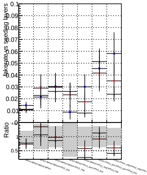
Fake rate vs. DOM V0001 R0000000001 Global CMSSW ckfPU50 RECO DOM V0001 R0000000001 Global CMSSW InkFIRPU50 LowPtQuad RECO DOM V0001 R0000000001 Global CMSSW LowPtOnoclean RECO
