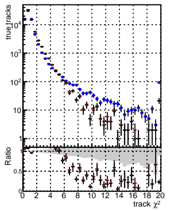
N of reco track vs. \chi^2 Global_CMSSW_cxFW50_RECO Global_CMSSW_mkfFW50_lowPtQuad_RECO DGM_V0001 R0000000000 DGM_V0000 R0000000000
