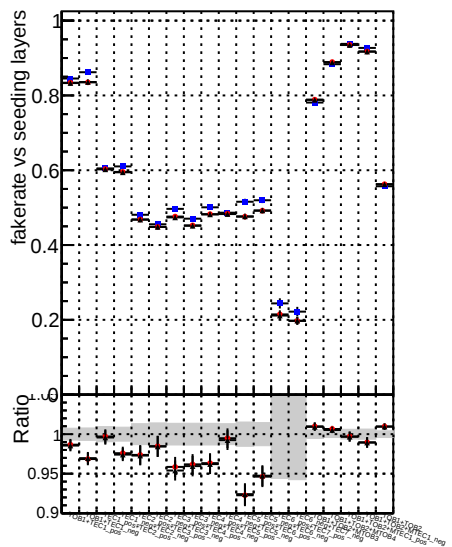
Fake rate vs. DOM V0001 R0000000001 Global CMSSW_ckptPU50_RECO DOM V0001 R0000000001 Global CMSSW_ckptPU50_RECO DOM V0001 R0000000001 Global CMSSW_ckptPU50_RECO DOM V0001 R0000000001 Global CMSSW_ckptPU50_RECO
