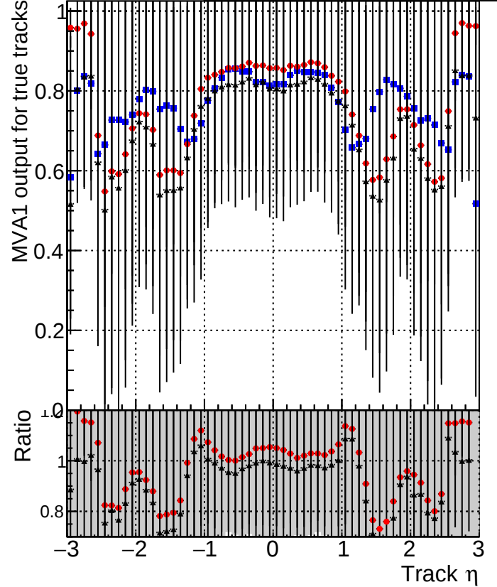
MVA1 of associated tracks (recoToSim) vs. track \eta ■ DQM_V0001_R0000000001_Global_CMSSW_ckfPU50_RECO ◆ DQM_V0001_R0000000001_Global_CMSSW_mkFitPU50LowPtQuad_RECO ★ DQM_V0001_R0000000001_Global_CMSSW_LowptQnoclean_RECO
