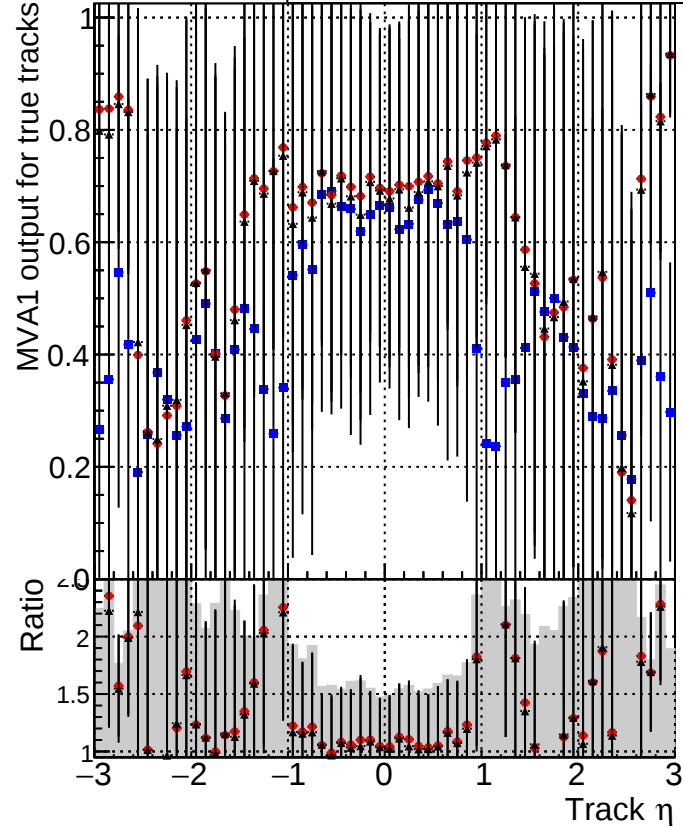
MVA1 of associated tracks (recoToSim) vs. track \eta ■ DQM_V0001_R000000001_Global_CMSSW_ckfPU50_RECO ● DQM_V0001_R000000001_Global_CMSSW_mkFitPU50LowPtQuad_RECO ▲ DQM_V0001_R000000001_Global_CMSSW_LowptQnoclean_RECO
