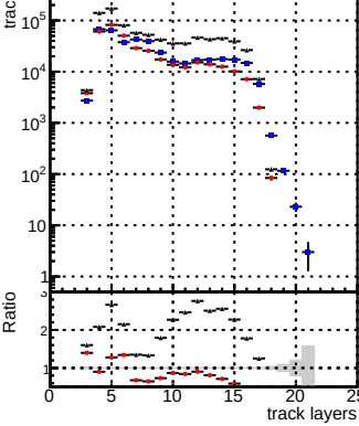
N of reco track vs layer
