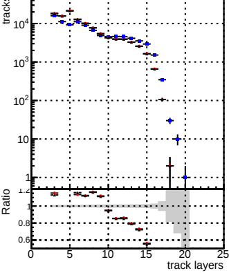
N of reco track vs track layers
