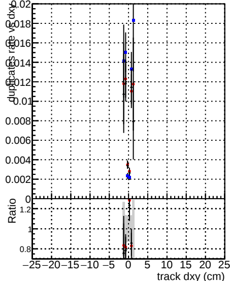
Global CMSSW ckfPU50 RECO Global CMSSW InFIRPU50 LowPtQuad RECO Global CMSSW LowPtOnoclean RECO
