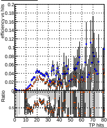
Efficiency vs hit Legend: DQM_V0001_R000000001_Global_CMSSW_ckfPU50_RECO DQM_V0001_R000000001_Global_CMSSW_mkFitPU50LowPtQuad_RECO DQM_V0001_R000000001_Global_CMSSW_LowptQnoSC_RECO DQM_V0001_R000000001_Global_CMSSW_LowptQnoDC_RECO
