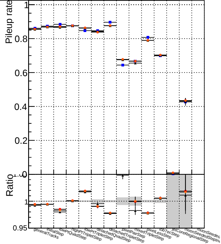
CMSSW_ckptPU50 RECO CMSSW_mkFitPU50LowPtQuad_RECO CMSSW_LowptQnoSC_RECO CMSSW_LowptQnoDC_RECO
