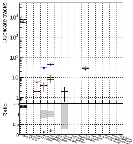
Number DQM V0001 R0000000001 Global CMSSW LowptQnoSC RECO RECO DQM V0001 R0000000001 Global CMSSW LowptQnoDC RECO DQM V0001 R0000000001 Global CMSSW LowptQnoDC RECO
