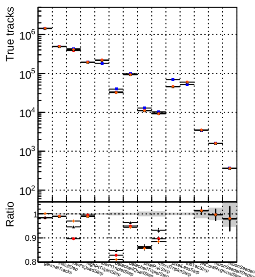
Number Legend QID Run Number Beam Detector Configuration —●— DQM_V0001 R000000001 Global CMSSW ckfPU50_RECO —●— DQM_V0001 R000000001 Global CMSSW mkFitPU50LowPtQuad_RECO —●— DQM_V0001 R000000001 Global CMSSW LowptQnoSC_RECO —●— DQM_V0001 R000000001 Global CMSSW LowptQnoDC_RECO
