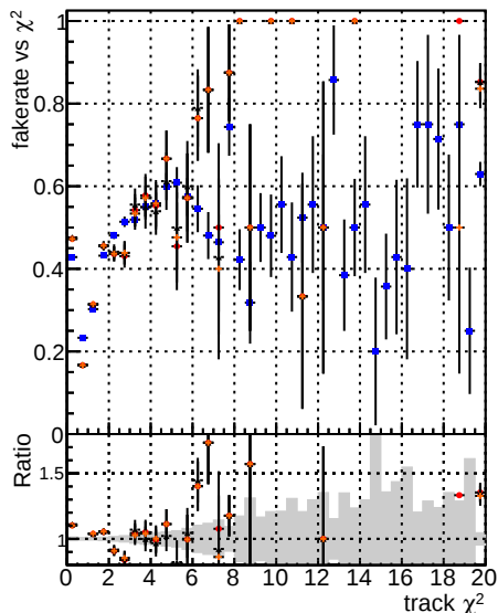
Fake rate vs. DGM_V0001 R000000000001 Global CMSSW skPH50_REC0 DGM_V0001 R000000000001 Global CMSSW skPH50_Quad_REC0 DGM_V0001 R000000000001 Global CMSSW LowPb50_8DC_REC0
