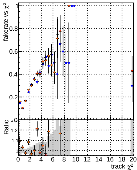
Fake rate vs. DOM V0001 R00000000001 Global GMSSW ckfPU50_RECQ LowPU50Quad_RECQ DOM V0001 R00000000001 Global CTMSSW LowPU50Quad_RECQ RECO DOM V0001 R00000000001 Global CTMSSW LowPU80C_RECQ RECO
