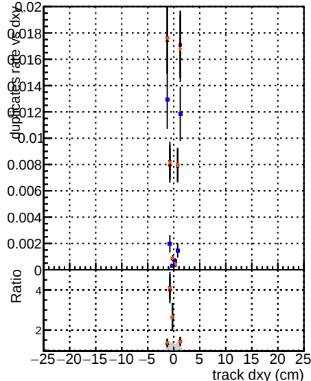
Global CMSSW skPH50 RECO CMSSW HighP50LoverQuad RECO CMSSW LowP50HDC RECO
