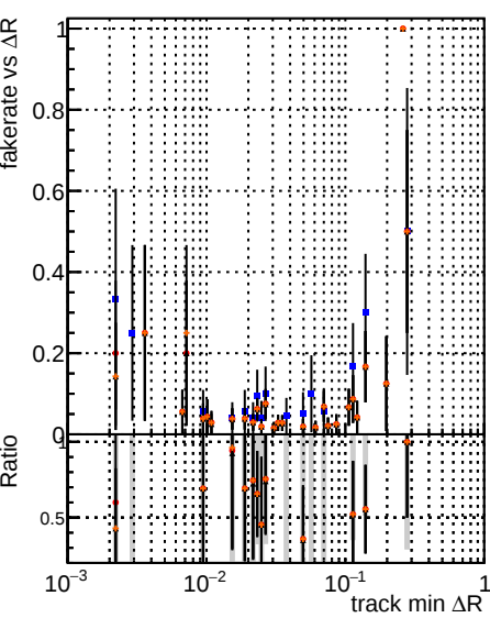
Fake rate vs \Delta R(\text{track, jet}) DQM V0001 R00000000001 Global CMSSW LFN50 RECO Global CMSSW LFN50 LowPileup RECO Global CMSSW LFN50 LowPileup RECO
