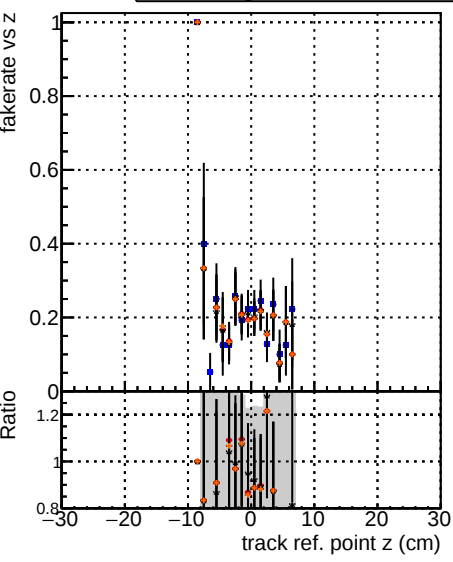
Fake rate vs v Global CMSSW PU50 RECO Global CMSSW PU50 LowPionDC Global CMSSW PU50 LowPionDC Global CMSSW PU50 LowPionDC
