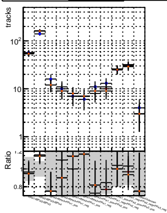
DOM V00001 R000000000001 Global CMSSW skPU50 RECO N of reco track vs. s
