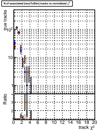
DOM V00001 R000000000001 Global CMSSW skPU50 RECO N of reco track vs. s
