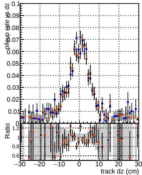
Global data CMSSW skPH50_500_Quad_RECO
