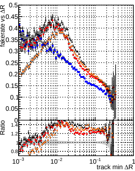
Fake rate vs \Delta R(\text{track, jet}) Global CMSSW PU50 RECO Global CMSSW PU50 RECO Global CMSSW PU50 RECO
