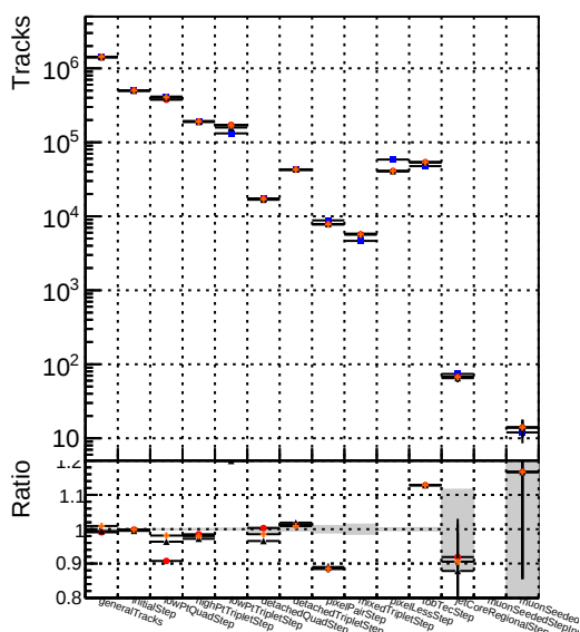
Number Legend QMC QMC ID QMC Type QMC Name —●— DQM_V0001 R000000001 Global CMSSW_ckfPU50_RECO —●— DQM_V0001 R000000001 Global CMSSW_mkFitPU50LowPtQuad_RECO —●— DQM_V0001 R000000001 Global CMSSW_LowptQnoSC_RECO —●— DQM_V0001 R000000001 Global CMSSW_LowptQnoDC_RECO
