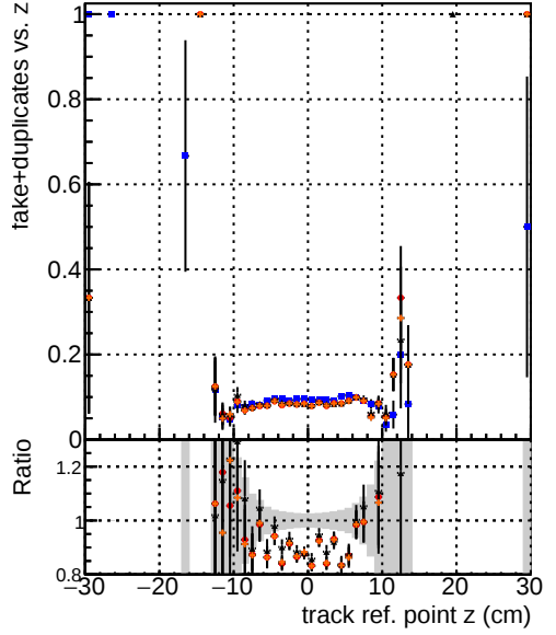
—●— DQM_V0001_R0000000001_Global_CMSSW_ckptPU50_RECO —●— DQM_V0001_R0000000001_Global_CMSSW_mkFitPU50LowPtQuad_RECO —●— DQM_V0001_R0000000001_Global_CMSSW_LowPtQnoSC_RECO —●— DQM_V0001_R0000000001_Global_CMSSW_LowPtQnoDC_RECO
