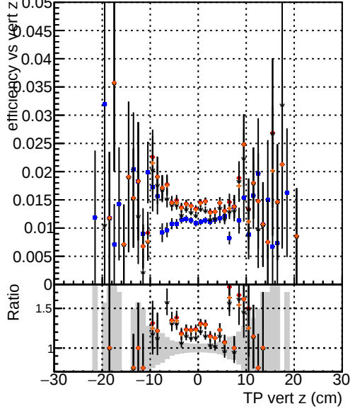
—●— DQM_V0001_R0000000001_Global_CMSSW_ckptPU50_RECO —●— DQM_V0001_R0000000001_Global_CMSSW_mkFitPU50LowPtQuad_RECO —●— DQM_V0001_R0000000001_Global_CMSSW_LowPtQnoSC_RECO —●— DQM_V0001_R0000000001_Global_CMSSW_LowPtQnoDC_RECO
