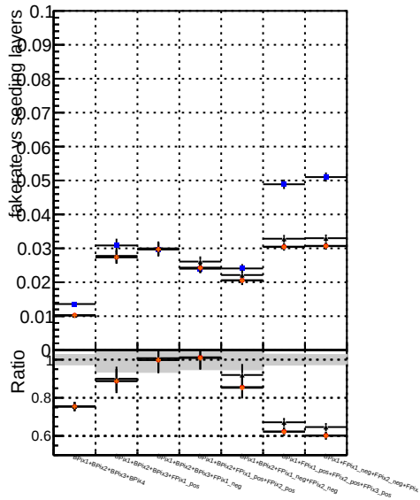
Fake rate vs. BQM V0001 BQM V0001 R00000000001 Global CMSSW skPH50 RECO BQM V0001 BQM V0001 R00000000001 Global CMSSW FullPH50 RECO BQM V0001 BQM V0001 R00000000001 Global CMSSW LowPileUp RECO BQM V0001 BQM V0001 R00000000001 Global CMSSW LowPileUp RECO
