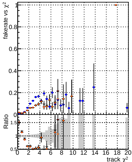
Fake rate vs. BQM V0001 BQM V0001 R00000000001 Global CMSSW skPH50 RECO BQM V0001 BQM V0001 R00000000001 Global CMSSW FullPH50 RECO BQM V0001 BQM V0001 R00000000001 Global CMSSW LowPileUp RECO BQM V0001 BQM V0001 R00000000001 Global CMSSW LowPileUp RECO
