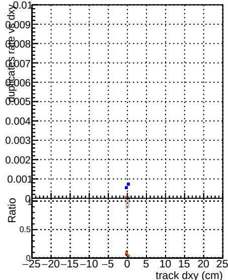
CMSSW LowbptOnoSC-RECO
