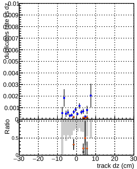
CMSSW LowbptOnoSC-RECO
