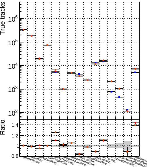
Number Symbol Model Method Model Method Model Method ● DQM V0001 R0000000001 Global CMSSW mkFitPU50 RECO ● DQM V0001 R0000000001 Global CMSSW mkFitPU50 RECO ● DQM V0001 R0000000001 Global CMSSW mkFitPU50LowPQuad RECO ● DQM V0001 R0000000001 Global CMSSW mkFitPU50LowPQuad-noBkwd RECO
