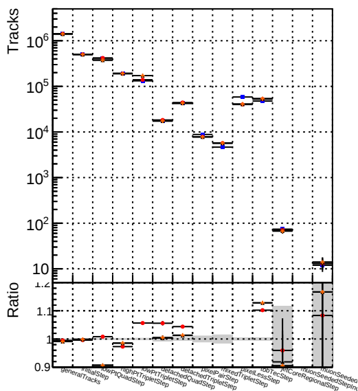
Number of tracks vs collection Legend: DQM_V0001_R000000001_Global_CMSSW_ckptPU50_RECO DQM_V0001_R000000001_Global_CMSSW_mkFitPU50_RECO DQM_V0001_R000000001_Global_CMSSW_mkFitPU50LowPtQuad_RECO DQM_V0001_R000000001_Global_CMSSW_mkFitPU50LowPtQuad-noBkwd_RECO
