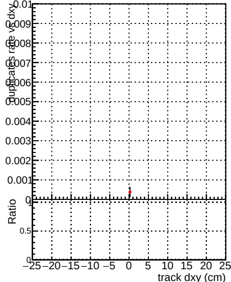
Legend for Fake rate vs d Legend for Duplicates Rate vs Dxy Legend for Pileup rate vs dxy B0M V0001 B000000000001 Global CMSSW skPU50 RECO B0M V0001 B000000000001 Global CMSSW skPU50 RECO B0M V0001 B000000000001 Global CMSSW skPU50 RECO B0M V0001 B000000000001 Global CMSSW skPU50 RECO B0M V0001 B000000000001 Global CMSSW skPU50 RECO B0M V0001 B000000000001 Global CMSSW skPU50 RECO
