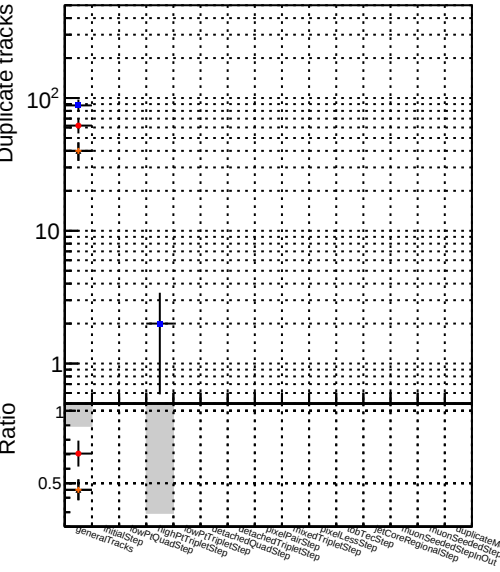
Number Symbol Label Region Model Reco ★ DQM_V0001_R0000000001 Global CMSSW_mkFitPU50LowPtQuad RECO ★ DQM_V0001_R0000000001 Global CMSSW_mkFitPU50LowPtQuad-noBkwd RECO
