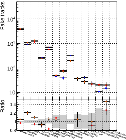
Number ★ DQM_V0001_R000000001 Global CMSSW_mkFitPU50LowPtQuad_RECO ★ DQM_V0001_R000000001 Global CMSSW_mkFitPU50LowPtQuad-noBkwd_RECO
