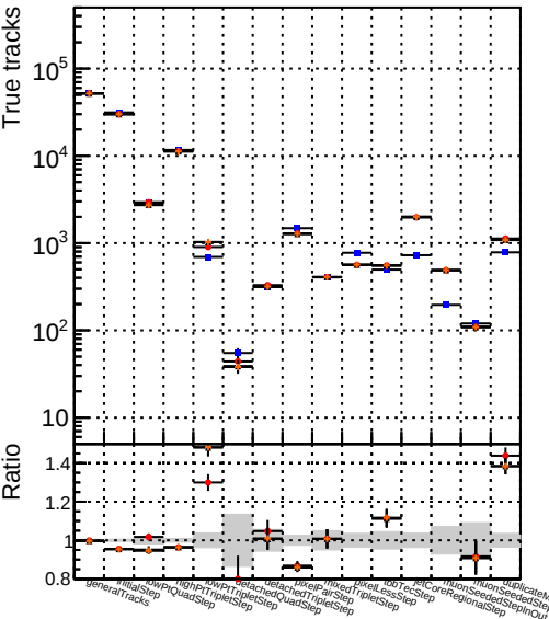
Number Model Dataset Model Dataset ● DOM_V0001 R0000000001 Global CMSSW CKtPU50 RECO ● DOM_V0001 R0000000001 Global CMSSW mkFitPU50 RECO ● DOM_V0001 R0000000001 Global CMSSW mkFitPU50LowPtQuad RECO ● DOM_V0001 R0000000001 Global CMSSW mkFitPU50LowPtQuad-noBkwd RECO
