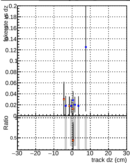
Fake rate vs d DGM V0001 D0000000001 C Global CMGSW SKIDU50 RECO DGM V0001 R0000000001 C Global LTM SWW HRPDU50 LOWPQuad RECO DGM V0001 R0000000001 C Global LTM SWW HRPDU50 LOWPQuad-noBkwd RECO
