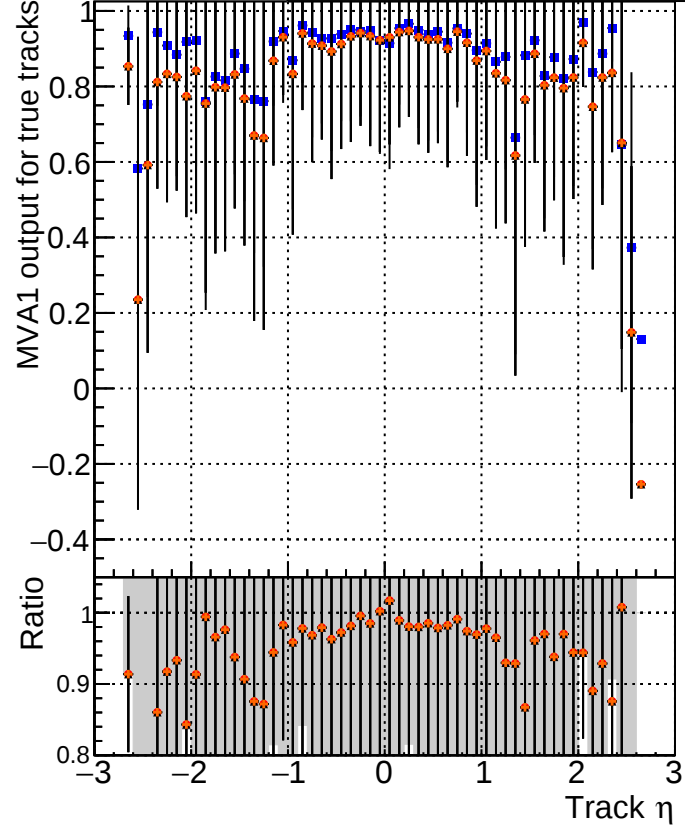
MVA1 of associated tracks (recoToSim) vs. track \eta ■ DQM_V0001_R0000000001 Global CMSSW_ckptPU50_RECO ● DQM_V0001_R0000000001 Global CMSSW_mkFitPU50_RECO ▲ DQM_V0001_R0000000001 Global CMSSW_mkFitPU50LowPtQuad_RECO ★ DQM_V0001_R0000000001 Global CMSSW_mkFitPU50LowPtQuad-noBkwd_RECO
