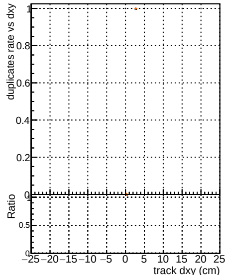
CMMSSWmkfFltpU50LowPtoQuad RECO
