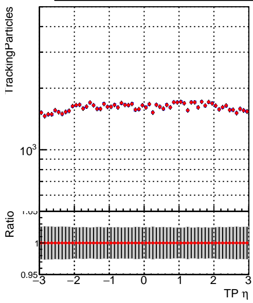
Legend: DQM_V0001_R0000000001_Global_CMSSW_ckf_RECO (blue squares), DQM_V0001_R0000000001_Global_CMSSW_mkFitOriginal_RECO (red circles)
