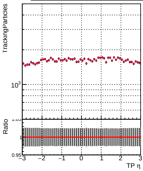
Legend: DQM_V0001_R000000001_Global_CMSSW_ckf_RECO (blue line), DQM_V0001_R000000001_Global_CMSSW_mkFitOriginal_RECO (red line)
