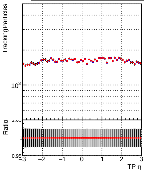
Legend: - Blue dots: DQM_V0001_R000000001_Global_CMSSW_ckf_RECO - Red dots: DQM_V0001_R000000001_Global_CMSSW_mkFitOriginal_RECO
