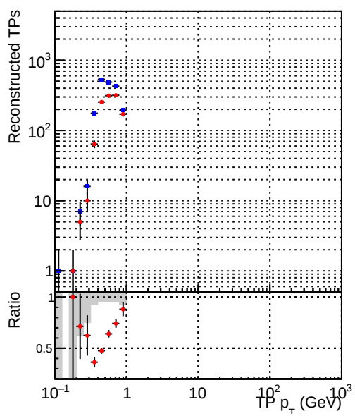
—•— DQM_V0001_R000000001_Global_CMSSW_ckf_RECO —•— DQM_V0001_R000000001_Global_CMSSW_mkFitOriginal_RECO
