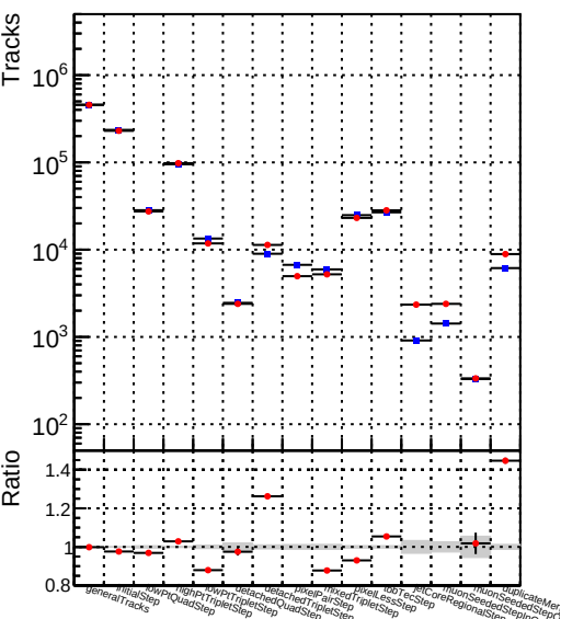
DQM_V0001_R000000001_Global_CMSSW_ckf_RECO
