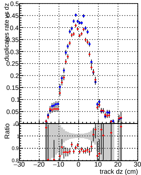
al_CMSSW_ckf_RECO al_CMSSW_mkFitOriginal_RECO
