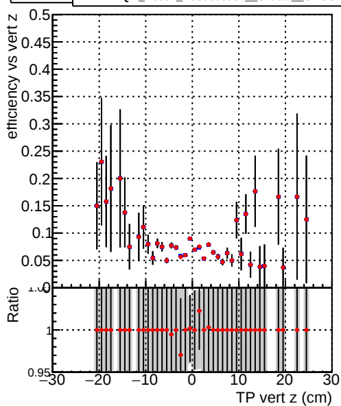
Efficiency vs vert z — DQM_V0001_R000000001_Global_CMSSW_ckf_RECO — DQM_V0001_R000000001_Global_CMSSW_mkFitOriginal_RECO
