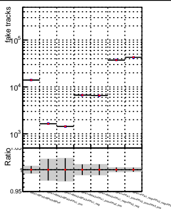
Global CMSSW_ckf_RECO Global CMSSW_mkFitOriginal_RECO
