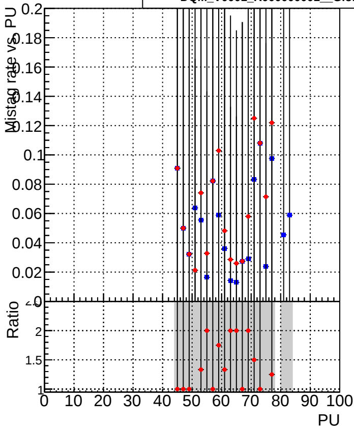
■ DQM_V0001_R000000001_Global_CMSSW_ckf_RECO ● DQM_V0001_R000000001_Global_CMSSW_mkFitOriginal_RECO
