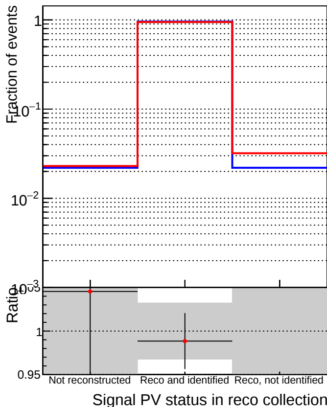
■ DQM_V0001_R000000001_Global_CMSSW_ckf_RECO ● DQM_V0001_R000000001_Global_CMSSW_mkFitOriginal_RECO
