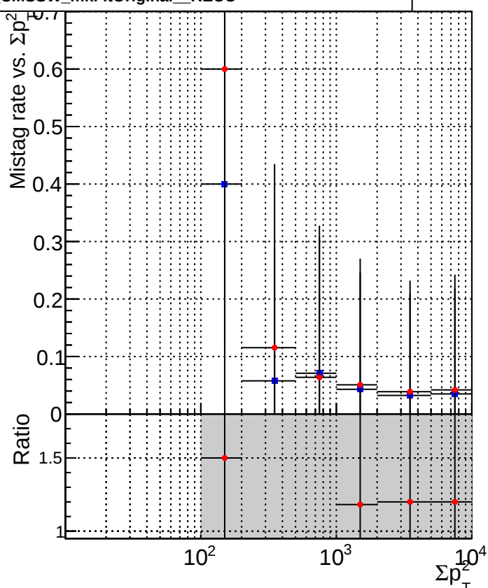
■ DQM_V0001_R000000001_Global_CMSSW_ckf_RECO ● DQM_V0001_R000000001_Global_CMSSW_mkFitOriginal_RECO
