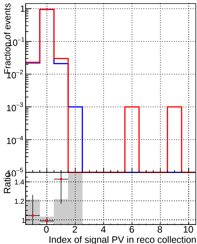
■ DQM_V0001_R000000001_Global_CMSSW_ckf_RECO ● DQM_V0001_R000000001_Global_CMSSW_mkFitOriginal_RECO
