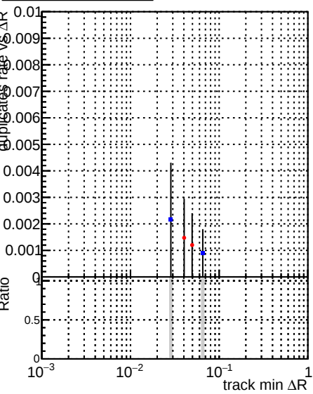
—•— DQM_V0001_R000000001_Global_CMSSW_ckf_RECO —•— DQM_V0001_R000000001_Global_CMSSW_mkFitOriginal_RECO
