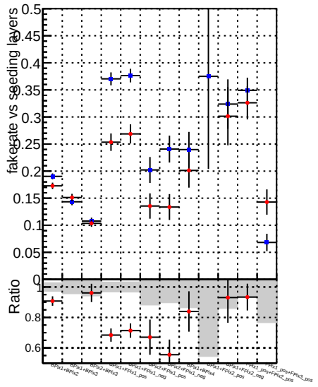
Fake rate vs. —●— DQM V0001 R0000000001 Global CMSSW_ckf RECO —●— DQM V0001 R0000000001 Global CMSSW_mkFitOriginal RECO
