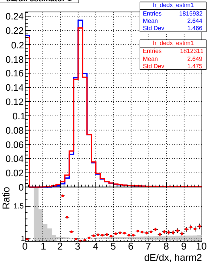
DQM_V0001_R000000001_Global_CMSSW_ckf_RECO DQM_V0001_R000000001_Global_CMSSW_mkFitOriginal_RECO
