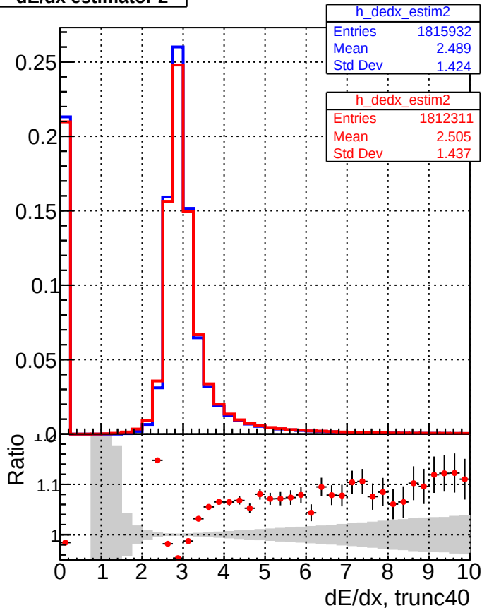
DQM_V0001_R000000001_Global_CMSSW_ckf_RECO DQM_V0001_R000000001_Global_CMSSW_mkFitOriginal_RECO
