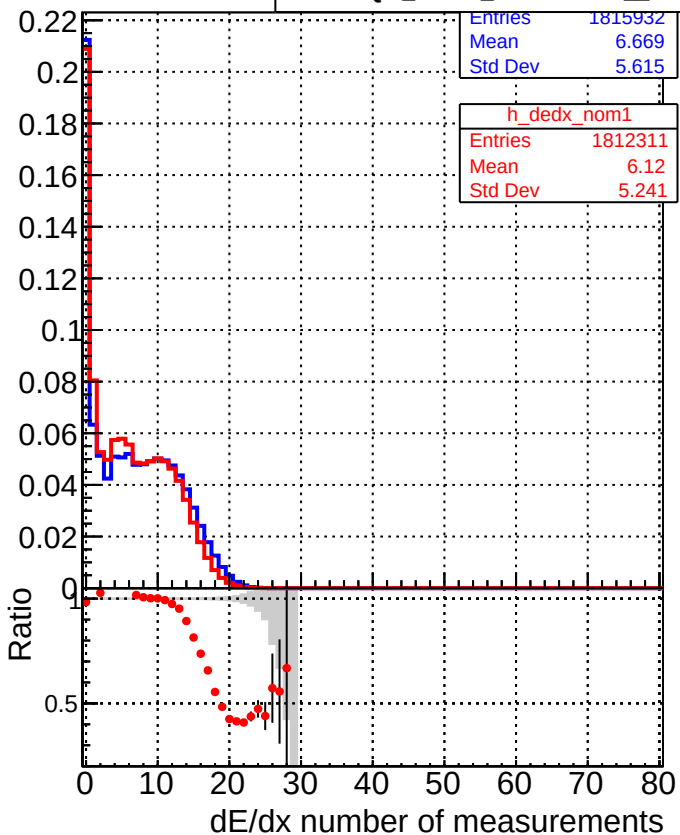
DQM_V0001_R000000001_Global_CMSSW_ckf_RECO DQM_V0001_R000000001_Global_CMSSW_mkFitOriginal_RECO
