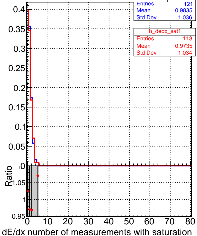
■ DQM_V0001_R000000001_Global_CMSSW_ckf_RECO ● DQM_V0001_R000000001_Global_CMSSW_mkFitOriginal_RECO
