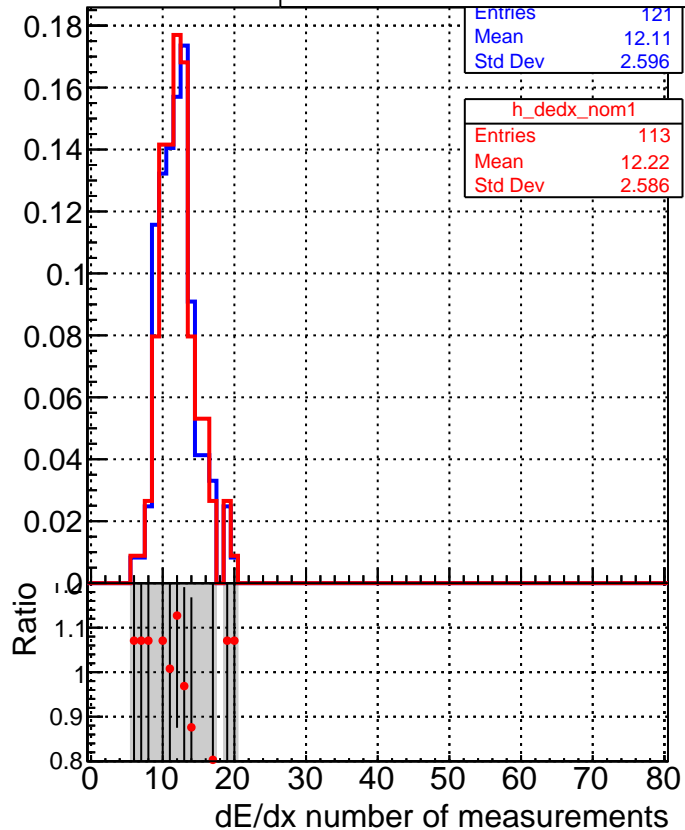
■ DQM_V0001_R000000001_Global_CMSSW_ckf_RECO ● DQM_V0001_R000000001_Global_CMSSW_mkFitOriginal_RECO
