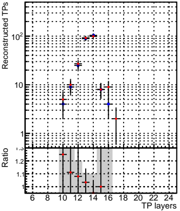
■ DQM_V0001_R000000001_Global_CMSSW_ckf_RECO ■ DQM_V0001_R000000001_Global_CMSSW_mkFitOriginal_RECO
