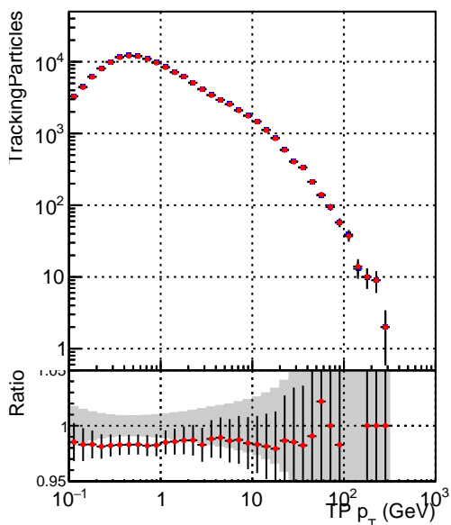
— DQM_V0001_R000000001_Global_CMSSW_ckf_RECO — DQM_V0001_R000000001_Global_CMSSW_mkFitOriginal_RECO
